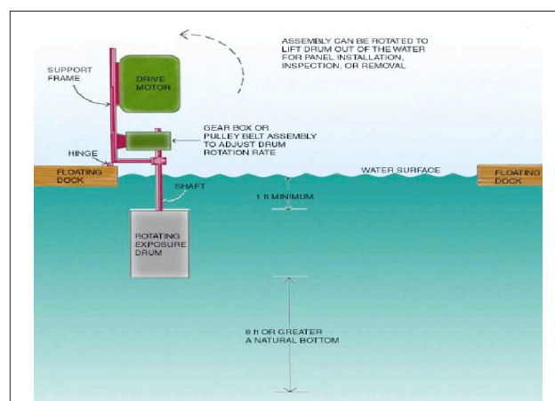
Figure 7. The above represents a diagrammatic representation of the rotating drum design for dynamic testing (ASTM D-4938).
