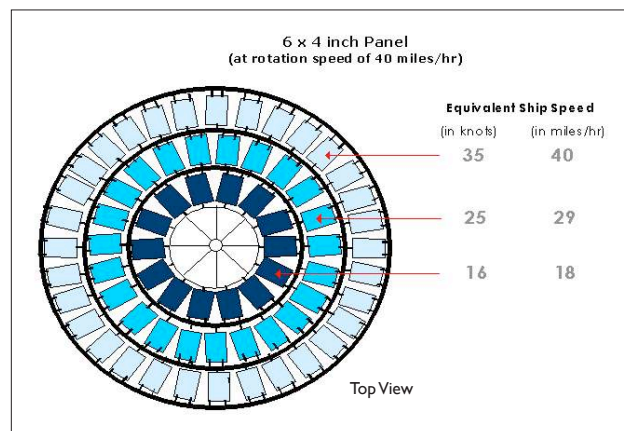
Figure 9. The positions of the 4 x 6 in panels on each 'disc'.
